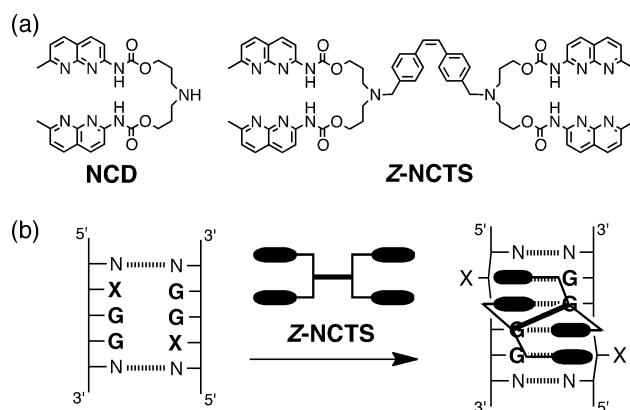
Figure 1. a) Chemical structures of NCD and Z-NCTS. b) Illustration of the binding of Z-NCTS to d(XGG)/d(XGG) (X = C, G, T, or A).
